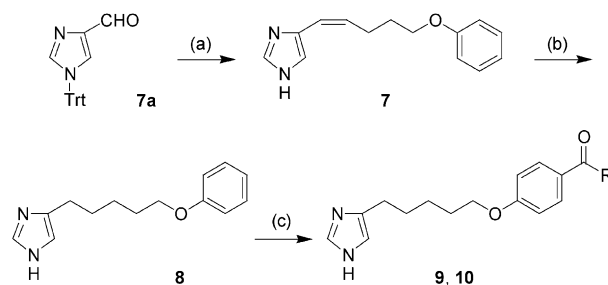
Scheme 2. Synthesis of 5-(1 H -imidazol-4-yl)pent(en)yl derivatives 7–10 . (a) (i): \text{PhO}(\text{CH}_2)_4\text{PPh}_3^+\text{Br}^- , \text{KOC}(\text{CH}_3)_3 , THF, 18 h; (ii) 2 N HCl, acetone, reflux, 1 h; (b) \text{H}_2 (10 bar), Pd/C, MeOH/2 N HCl, rt, 18 h; (c) corresponding acyl halide, \text{AlCl}_3 , nitrobenzene, rt, 3 days; R = \text{CH}_3 ( 9 ); R = \text{C}_2\text{H}_5 ( 10 ).
