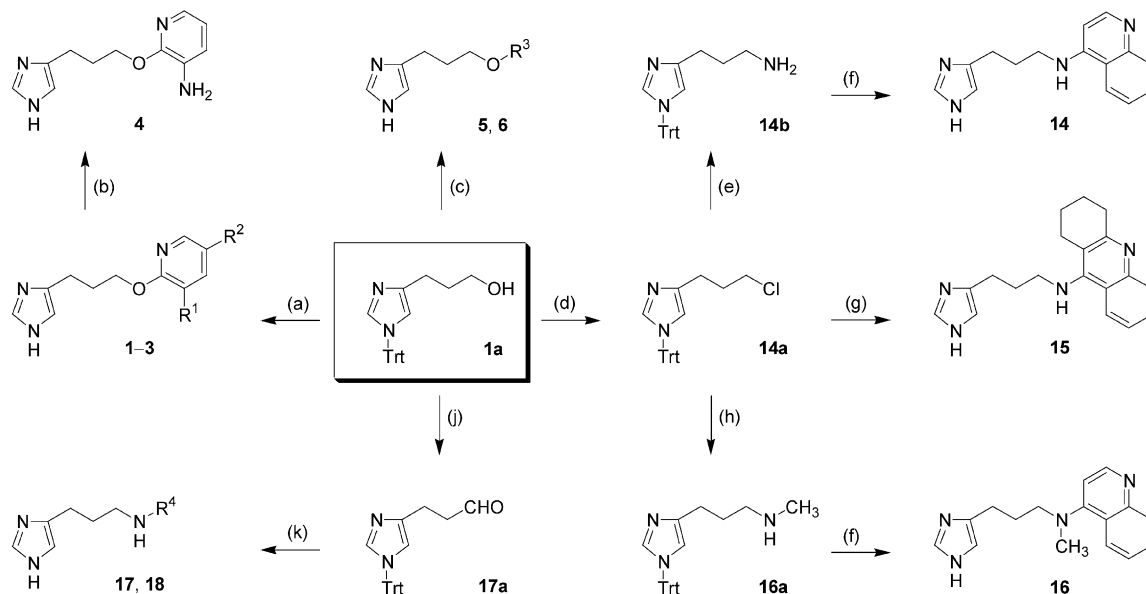
Scheme 1. Synthesis of 3-(1 H -imidazol-4-yl)propyl derivatives 1–6 and 14–18 . (a) (i) Corresponding chloropyridine, NaH, THF, 60 °C, 12 h; (ii) 2 N HCl, acetone, reflux, 2 h; (b) 2 only: \text{H}_2 (1 bar), Pd/C, rt, 18 h; (c) (i) corresponding phenol, \text{Ph}_3\text{P} , DEAD, THF, rt, 72 h; (ii) 2 N HCl, acetone, reflux, 1 h; (d) \text{SOCl}_2 , THF, rt, 2 h; (e) \text{NH}_3 (fl.), [\text{H}_3\text{C}(\text{CH}_2)_3]_4\text{NI} , \text{NH}_4\text{Cl} , EtOH, rt, 12 h → 60 °C, 24 h; (f) (i) 4-chloroquinoline, phenol, 140 °C, 12 h; (ii) 2 N HCl, THF, reflux, 2 h; (g) (i) 1,2,3,4-tetrahydroacridin-9-amine, NaH, [\text{H}_3\text{C}(\text{CH}_2)_3]_4\text{NI} , DMF, 140 °C, 12 h; (ii) 2 N HCl, THF, reflux, 2 h; (h) \text{H}_3\text{CNH}_2 , KOH, KI, EtOH/ \text{H}_2\text{O} , reflux, 12 h; (j) (\text{COCl})_2 , DMSO, (\text{H}_5\text{C}_2)_3\text{N} , \text{CH}_2\text{Cl}_2 , –55 °C → rt, 4 h; (k) (i) corresponding aminoquinoline, \text{Na}(\text{CH}_3\text{CO}_2)_3\text{BH} , \text{H}_3\text{CCOOH} , 1,2-dichloroethane, rt 3 days; (ii) 2 N HCl, acetone, reflux, 1 h; R 1 , R 2 = H ( 1 ); R 1 = NO 2 , R 2 = H ( 2 ); R 1 = H, R 2 = NO 2 ( 3 ); R 3 = 4-(3-nitropyridin-2-yl)aminophenoxy ( 5 ); R 3 = 5-nitroquinolin-8-yloxy ( 6 ); R 4 = 2-methylquinolin-6-yl ( 17 ); R 4 = quinolin-6-yl ( 18 ); Trt = triphenylmethyl.
