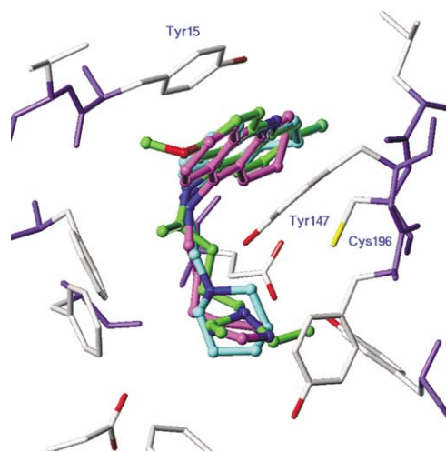
Figure 2. HMT inhibitor interactions: The acridine and tetrahydroacridine ring system, respectively, is sandwiched between Tyr147 and Cys196 on the one side and Tyr115 on the other. The cationic head of the compounds is interacting with several aromatic residues located at the bottom of the binding pocket.
