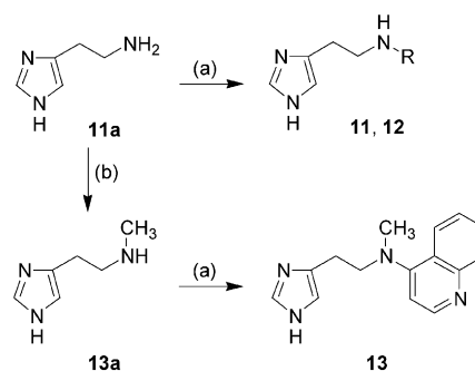
Scheme 3. Synthesis of 2-(1 H -imidazol-4-yl)ethyl derivatives 11–13 . (a) Corresponding aryl chloride, phenol, 140 °C, 12 h; (b) (i) N,N' -carbonyldiimidazole, 100 °C→120 °C, 1 h; (ii) LiAlH 4 , THF, reflux, 2 h; R = quinolin-4-yl ( 11 ); R = 1,2,3,4-tetrahydroquinolin-9-yl ( 12 ).
