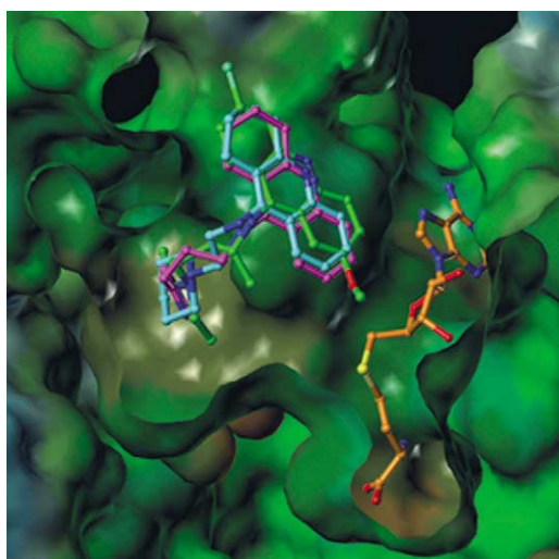
Figure 1. HMT inhibitor interactions: Comparison between the experimentally observed structure of quinacrine (green) and the docked compounds imidazole 15 (magenta) and FUB 854 (cyan). The co-crystallized reaction product S -adenosylhomocysteine is colored orange. The protein surface is colored according to the hydrophobic potential (blue = hydrophilic areas, brown = hydrophobic areas, calculated with the MOLCAD software). 45
