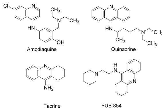
Chart 1. Amodiaquine, quinacrine, and tacrine, inhibitors of HMT, and FUB 854, a prototype HMT inhibitor with combined histamine H_3 receptor antagonist potency.
